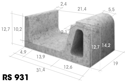
RS 931 Base
