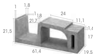
RS 911 Base
