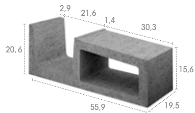
RS 921 Base
