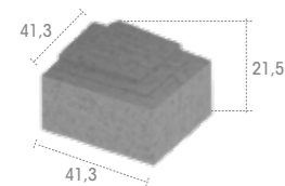
RS 918 Esquina exterior Outside corner Angle extérieur
