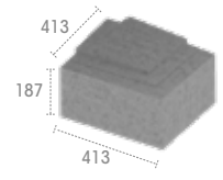
RS 918 Esquina exterior Outside corner Angle extérieur
